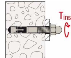
6: Apply T_{inst}
