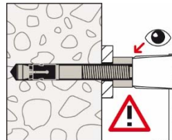
5.2: Check offset
